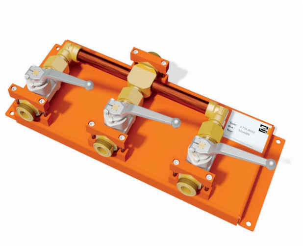
4 x DN20 without couplings Order no.: 3-718-R002
