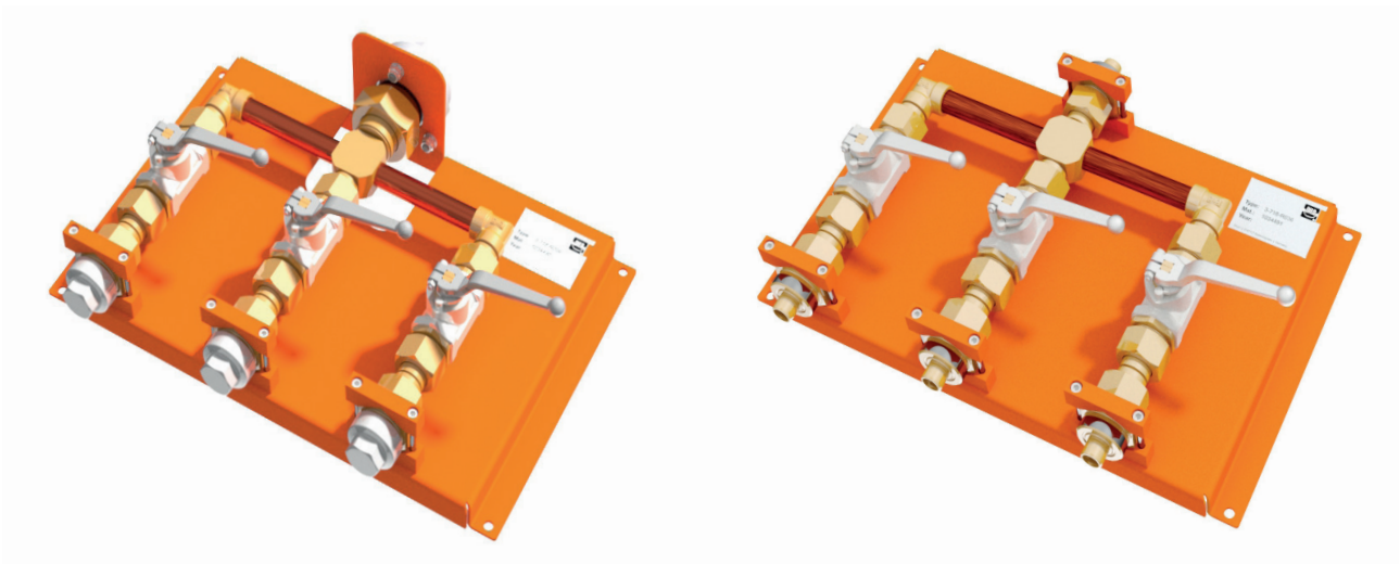
3 x DN20 / 1 x DN40 Order no.: 3-718-R006
